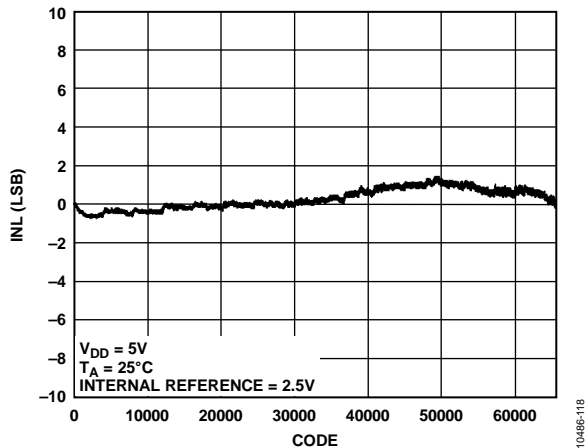
Figure 13. AD5696R INL
