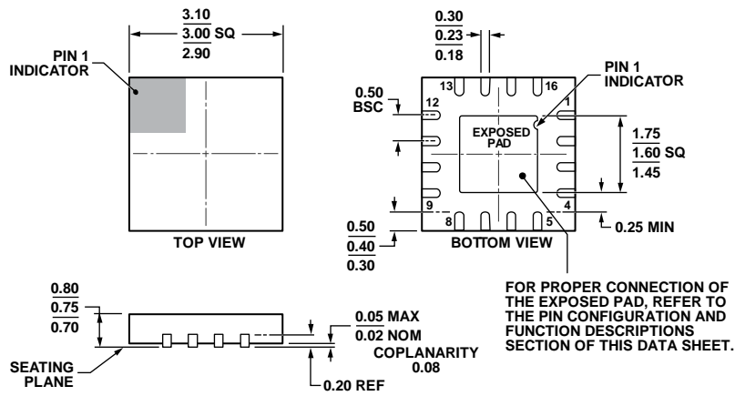
COMPLIANT TO JEDEC STANDARDS MO-220-WEED-6. Figure 61. 16-Lead Lead Frame Chip Scale Package [LFCSP_WQ] 3 mm x 3 mm Body, Very Very Thin Quad (CP-16-22) Dimensions shown in millimeters
