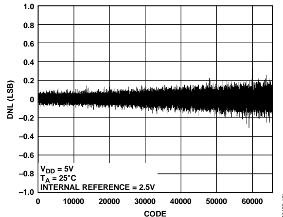
Figure 16. AD5696R DNL
