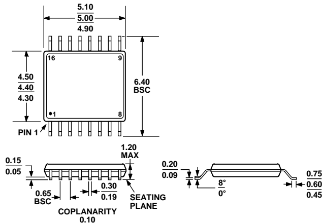
COMPLIANT TO JEDEC STANDARDS MO-153-AB Figure 62. 16-Lead Thin Shrink Small Outline Package [TSSOP] (RU-16) Dimensions shown in millimeters
